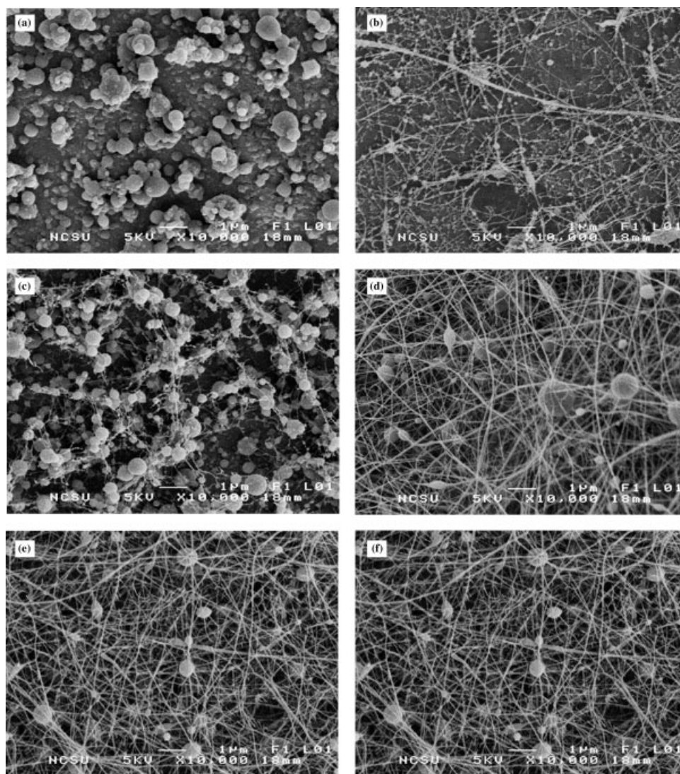
Figure 3 Effect of molecular weight and concentration on morphology of electrospun fibers. Low M_w nylon-6 10 wt % (a) and 15 wt % (b); medium M_w nylon-6 10 wt % (c) and 15 wt % (d); high M_w nylon-6 10 wt % (e), and 15 wt % (f) (All samples at 15kV, 15 \mu L/min, 15 cm).
