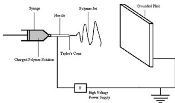
Figure 1 Typical electrospinning setup.
